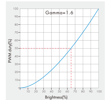
Logarithmic dimming curve
